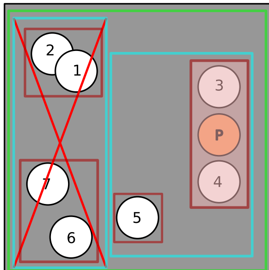
Figure 184: Querying an AABB-tree (3/3)
